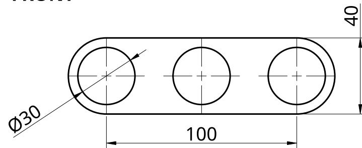
FRONT
